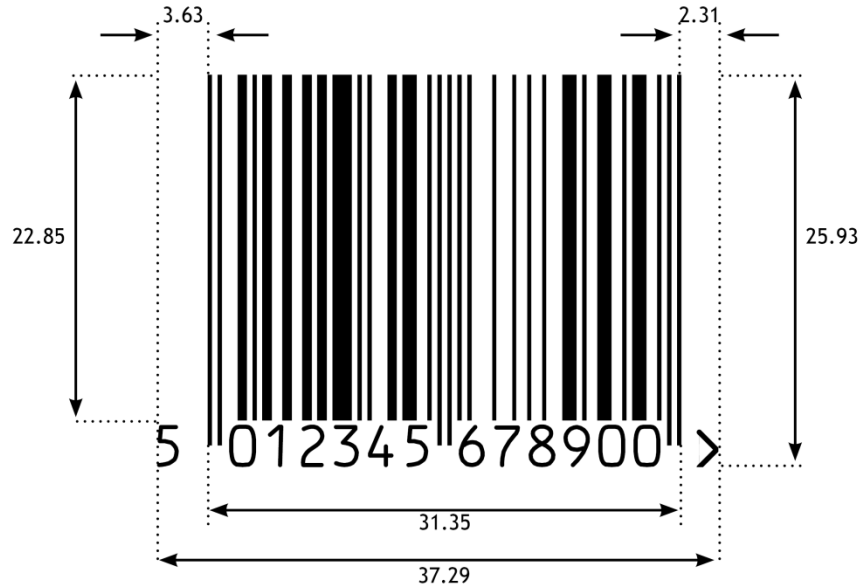
Figure 5.2.6.6-1. EAN-13 barcode
